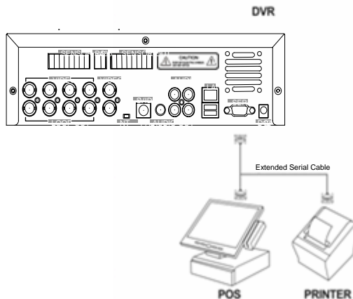
DVR & POS CONNECTION # POS : 1
